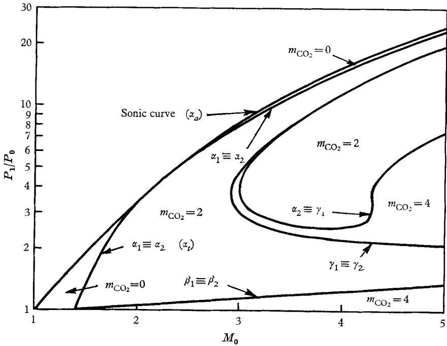
FIGURE 10. Multiple root lines and other critical curves for the air- \text{CO}_2 interface.
