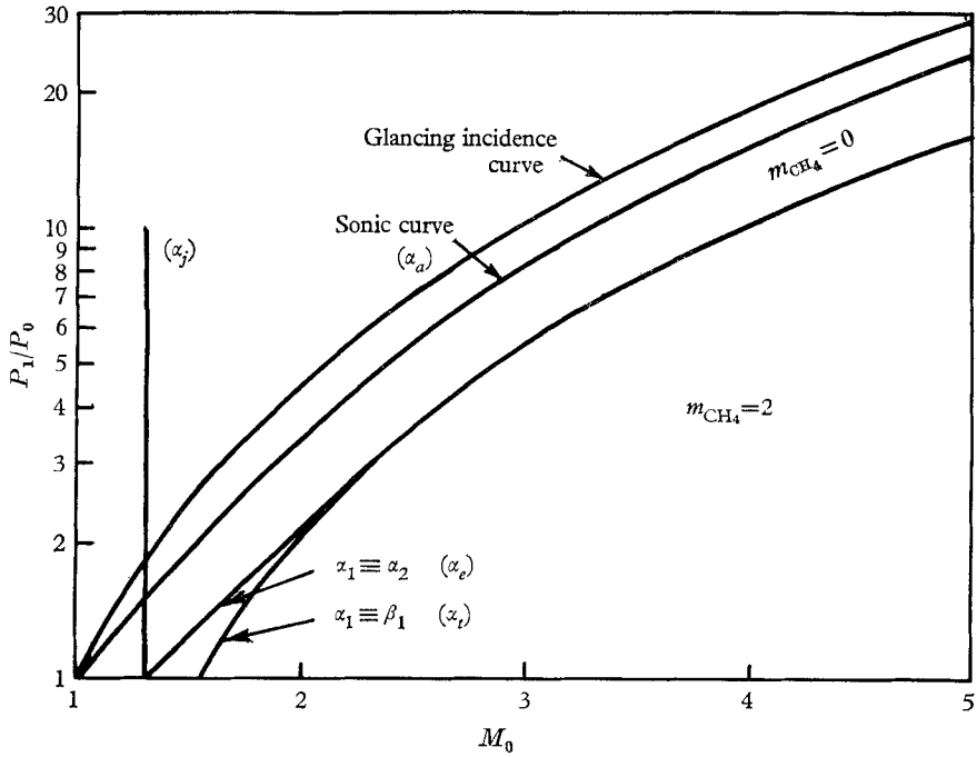
FIGURE 9. Multiple root lines and other critical curves for the air- \text{CH}_4 interface.
