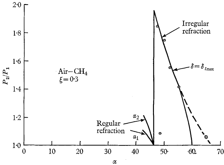
FIGURE 6. Theoretical and experimental results for irregular shock-wave refraction with \xi = 0.3 . —, three-shock theory; O, Jahn's experimental data; ---, curve of best fit through Jahn's data.
