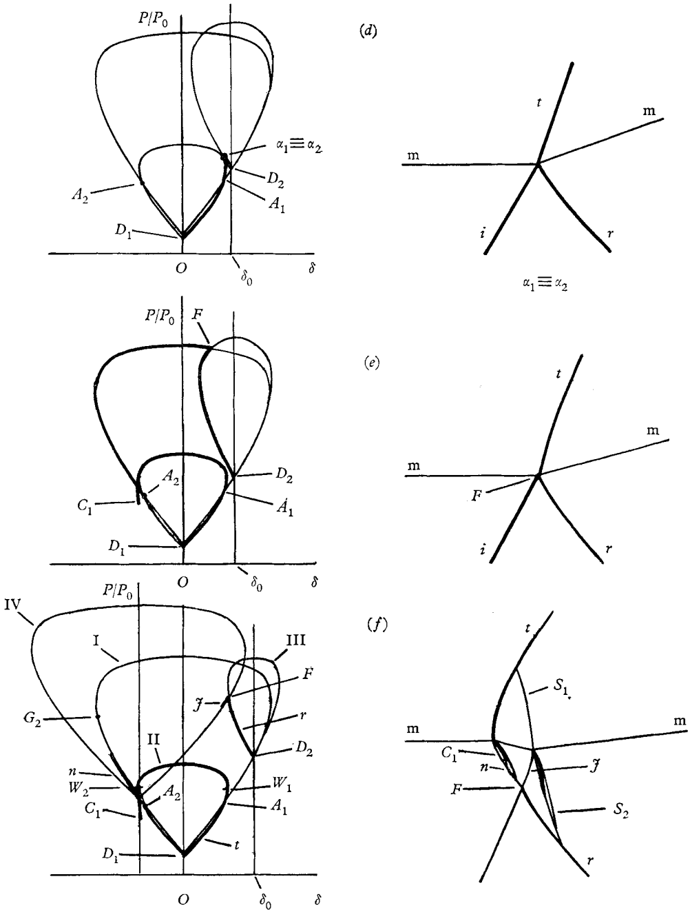
FIGURE 12. Sequence of events resulting from the displacement of polar III from polar I for the refraction of a plane shock i at an air-methane interface in the Mach-number range 1.55 \leq M_0 \leq 2.25 .
