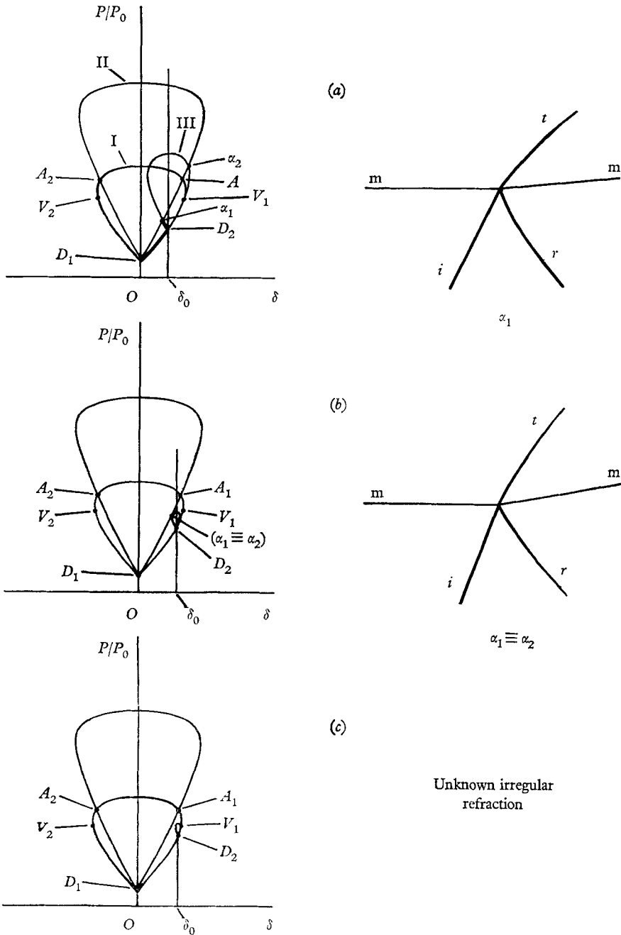
FIGURE 16. Sequence of events resulting from the displacement of polar III from polar I for the refraction of a plane shock i at an air-carbon dioxide interface in the Mach-number range 2.5 \leq M_0 \leq 2.92 .
