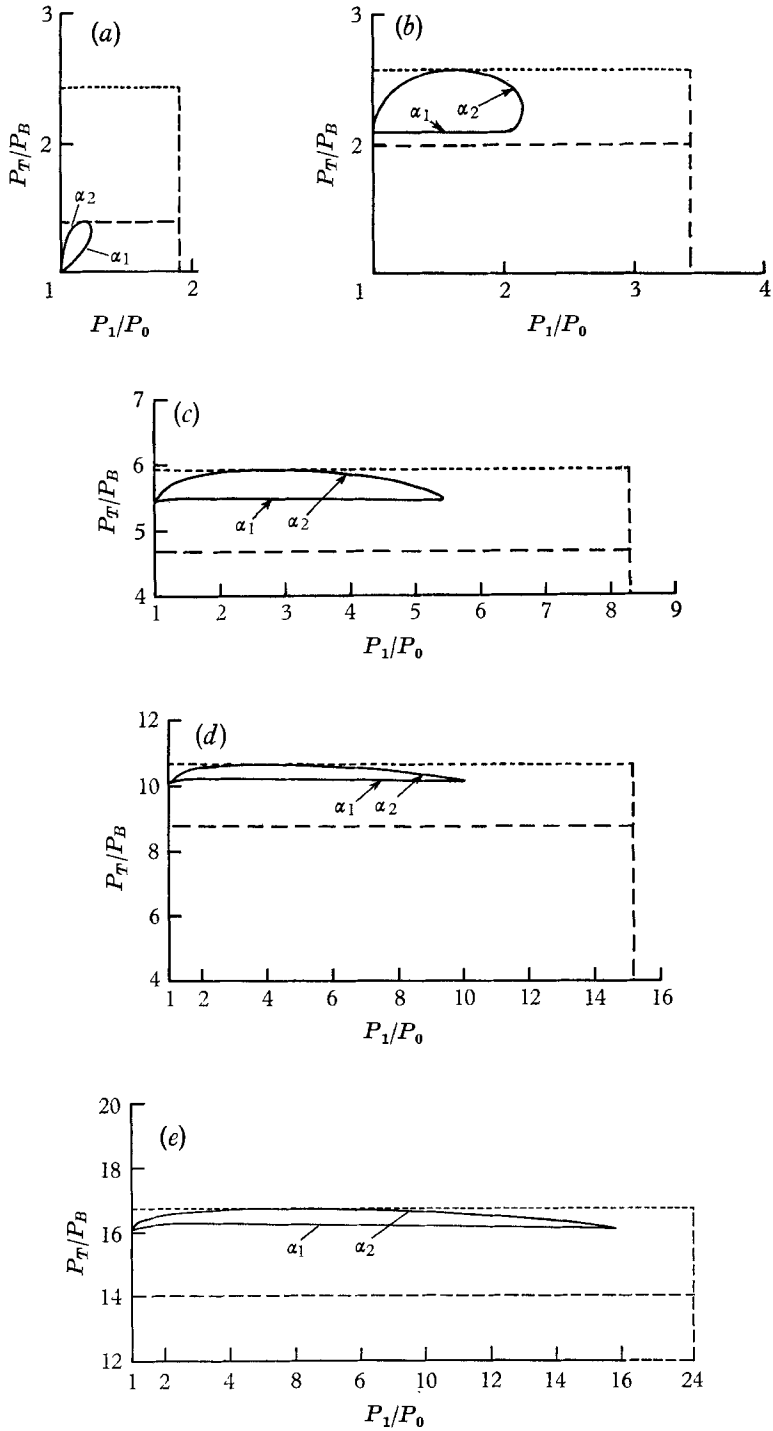
FIGURE 7. Physically significant roots of the polynomial equation for the regular refraction of a plane shock at the air- \text{CH}_4 interface. —, polynomial root line; ---, sonic line; ----, normal shock line. (a) M_0 = 1.5 ; (b) M_0 = 2.0 ; (c) M_0 = 3.0 ; (d) M_0 = 4.0 ; (e) M_0 = 5.0 .
