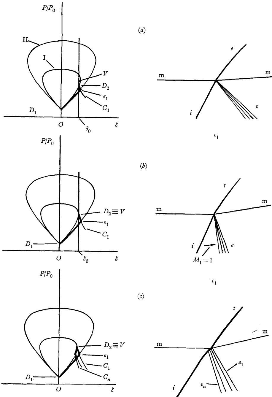
FIGURE 14. Sequence of events resulting from the displacement of the characteristic C_1 from the point D_1 for the refraction of a plane shock at an air-carbon dioxide interface in the Mach-number range M_0 \leq 1.38 .
